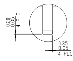
DETAIL G SCALE 4:1
