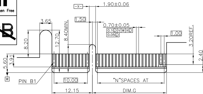
I/O PANEL DIRECTION Recommended GOLD FINGER(B SIDE VIEW)
