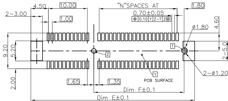
SOLDER PAD RECOMMEND P.C.B LAYOUT(COMPONENT SIDE)
