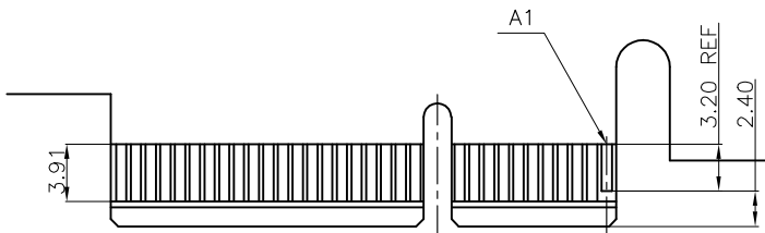
I/O PANEL DIRECTION Recommended GOLD FINGER(A SIDE VIEW)
