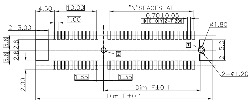
SOLDER PAD RECOMMEND P.C.B LAYOUT (COMPONENT SIDE) DEFAULT TOLERANCES: ±0.05; PCB THICKNESS: 1.2mm
