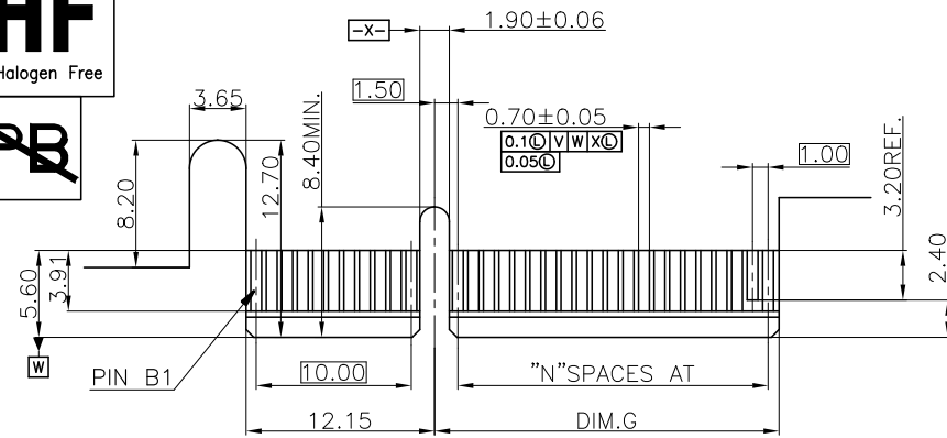
Recommended GOLD FINGER(B SIDE VIEW)
